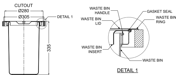
Stainless Steel Lid and 12 Litre Synthetic Bin
